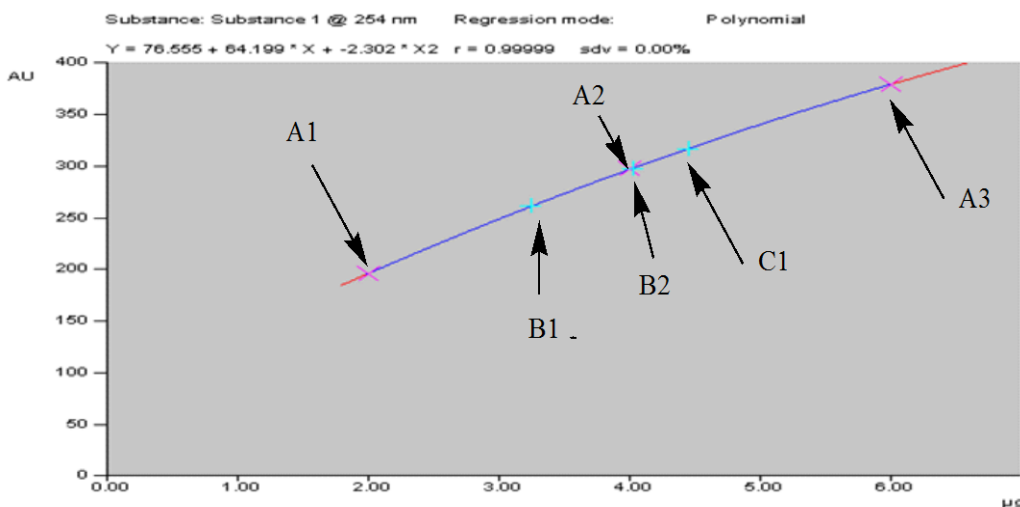
Figure 2: Polynomial regression curve graph via height of standard reference TQ (A1, A2, A3: three concentrations 2 \mu g, 4 \mu g, 6 \mu g). Unknown concentrations of: the methanol extract of NSWS B1 (60 \mu l), B2 (80 \mu l) and NSPO C1 (60 \mu l) showing the densitometric concentration of the unknown obtained after developing the TLC and scanning on the HPTL scanner III on the x-axis with pink color.
