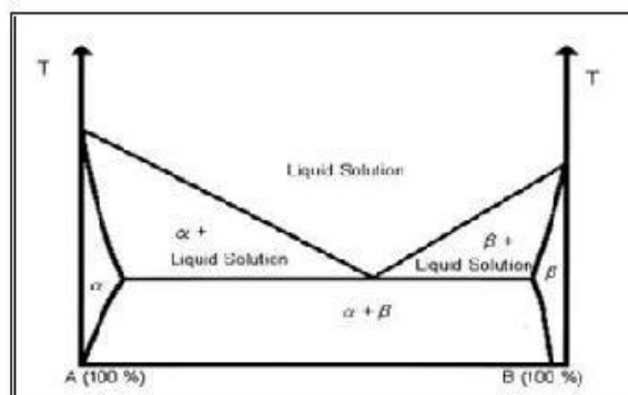
Fig. 2 Phase diagram for a discontinuous solid solution
