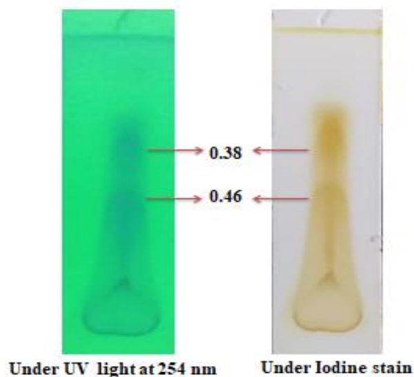
Figure.3: Active Compounds separated by Thin Layer Chromatography
