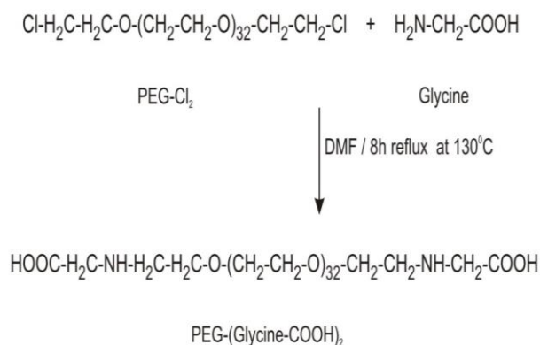
Scheme 2: Covalent binding of Glycine to PEG - Cl 2
