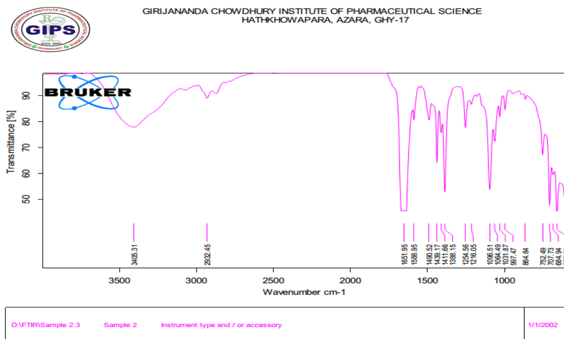
Figure 4: FTIR of PEGCl 2 -Glycine
