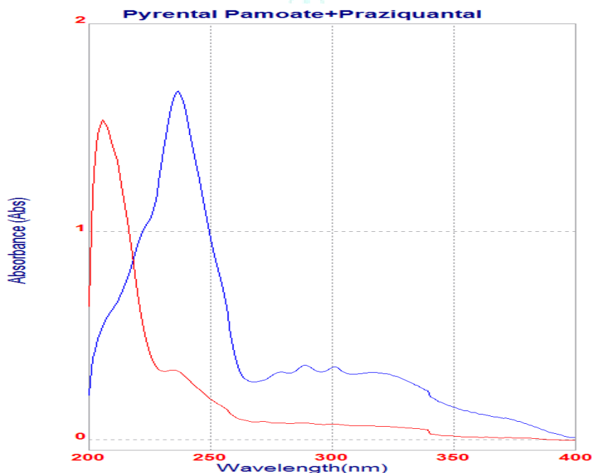
Fig. 3.Wavelength of Praziquantel and Pyrantele pamoate
