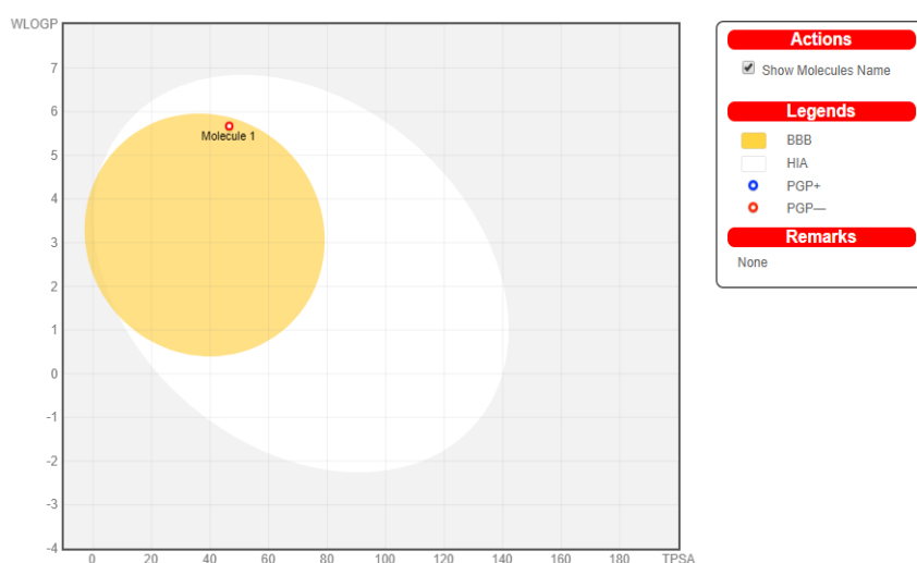
Figure 2: Molecule falling in egg's yolk is predicting the molecule is able to penetrate through the blood brain barrier.
