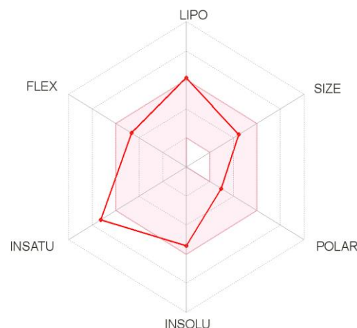
Figure 1: The bioavailability radar of TUG-891 using Swiss ADME predictor.
