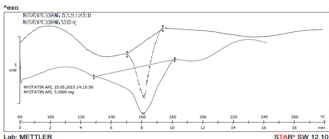
Figure 8.8: Comparative DSC graph of Microsphere of Nystatin
