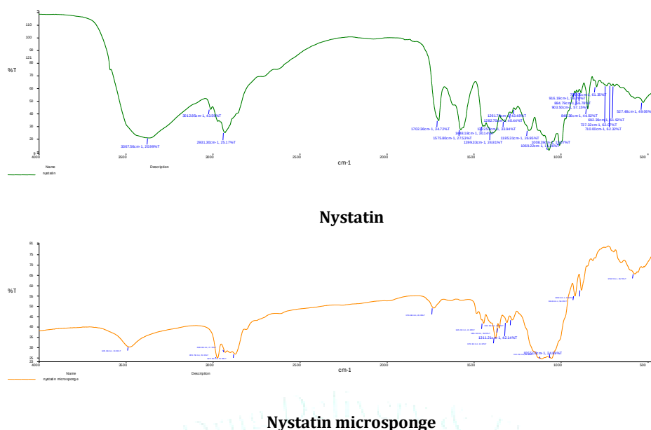
Figure 8.7: Comparative FTIR Spectra of Nystatin & microsphere
