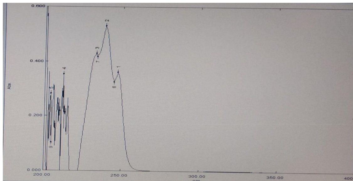
Figure 3: \lambda max of simvastatin
