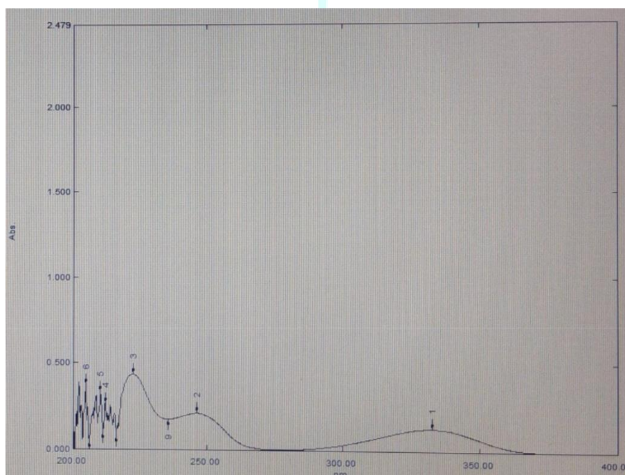
Figure 4: \lambda max of labetalol
