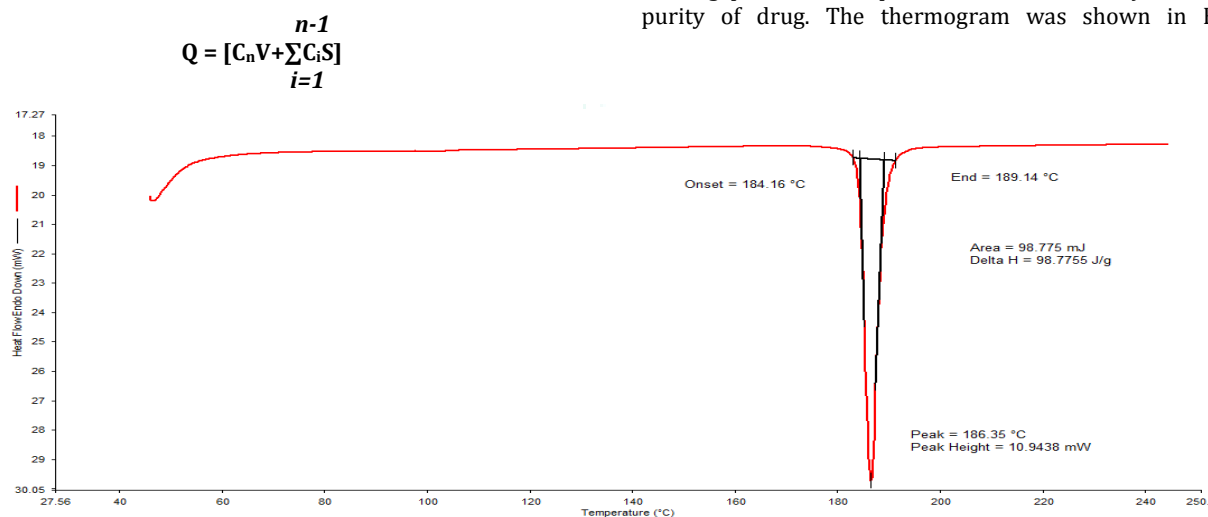
Figure 1: DSC thermogram of clozapine (CZP) pure drug
