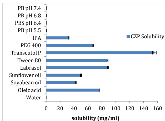
Figure 2: Solubility of clozapine in different solvents
