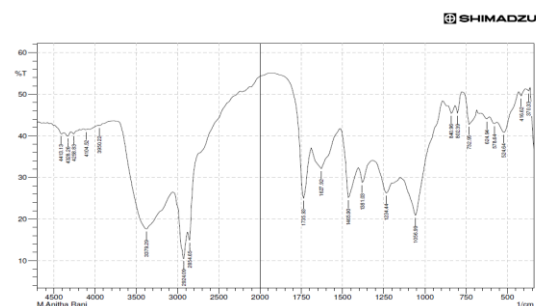
Figure 8: IR of Metformin, cholesterol and lecithin
