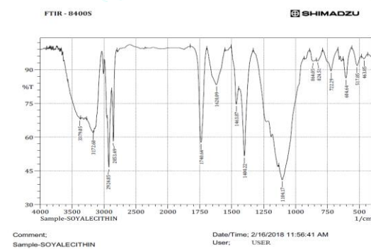
Figure 4: FT – IR of lecithin
