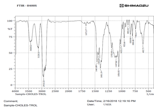
Figure 3: FT – IR of cholesterol
