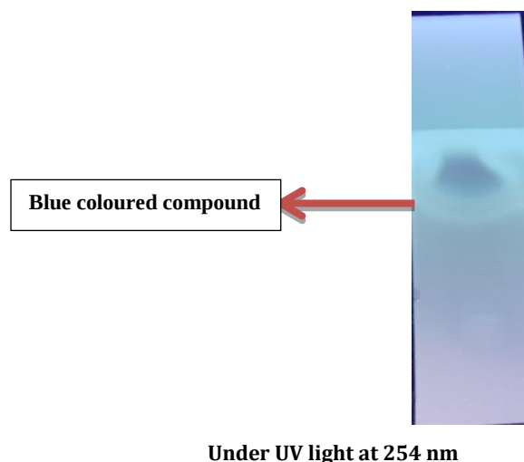
Figure 2: Separation of active Compounds by Thin Layer Chromatography
