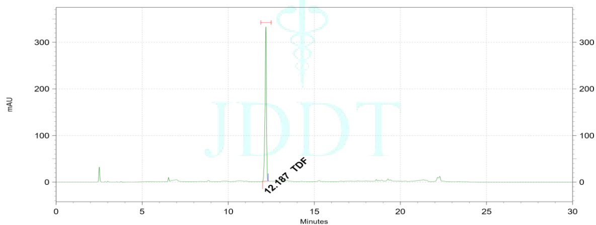
Figure 4: Chromatogram of Tenofovir disoproxil fumarate working standard
