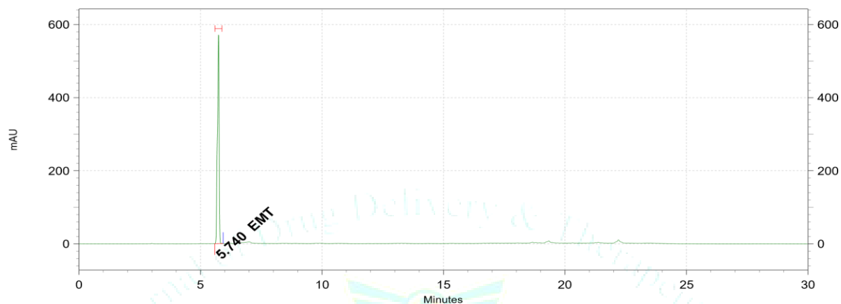
Figure 3: Chromatogram of Emtricitabine working standard
