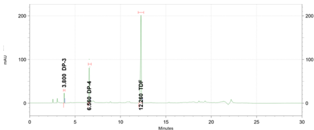
Figure 16: Chromatogram of acid hydrolysis of Tenofovir disoproxil fumarate
