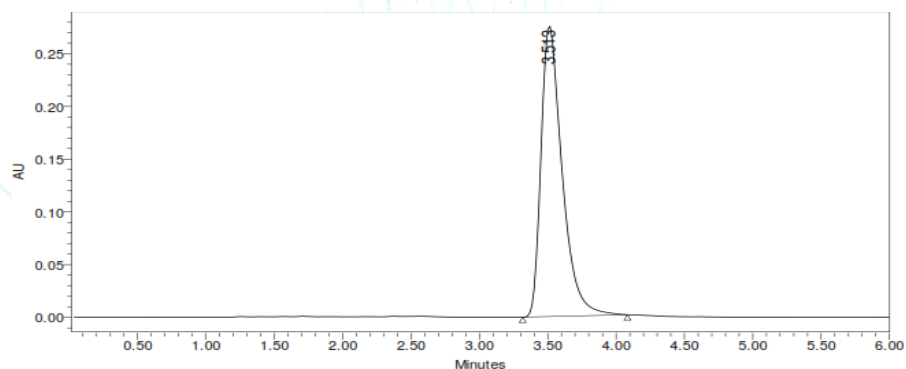
Figure 2a: Optimized Chromatogram (BortezomibStandard)
